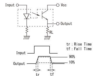
*1 Switching Time Measurement Circuit
