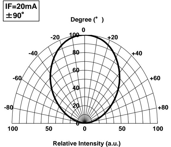
Directivity
