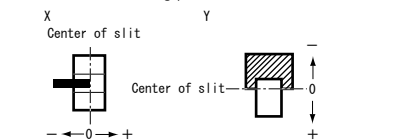
*2 Method of measuring position detection characteristic
