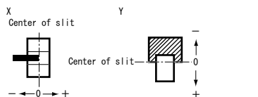
*2 Method of measuring position detection characteristic
