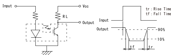
*1 Switching Time Measurement Circuit
