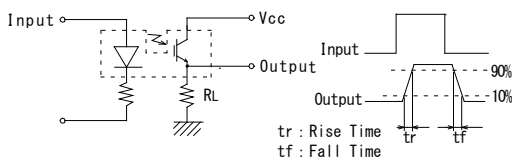
*1 Switching Time Measurement Circuit
