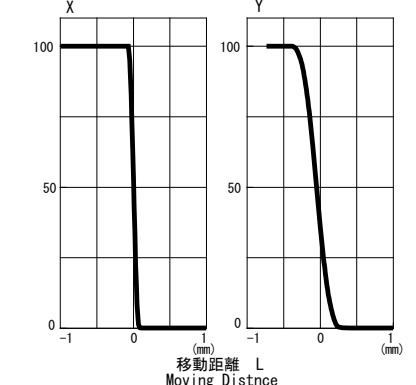
*2 Method of Measuring Position Detection Characteristic
