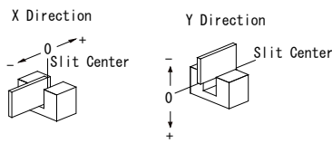
*2 Method of Measuring Position Detection Characteristic
