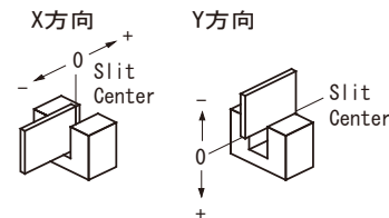
*2 Method of Measuring Position Detection Characteristic
