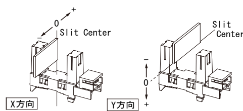
*2 Method of Measuring Position Detection Characteristic
