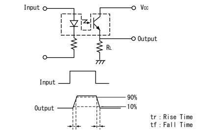
*1 Switching Time Measurement Circuit
