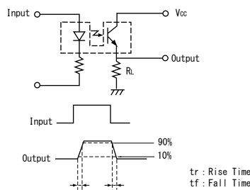
*1 Switching Time Measurement Circuit
