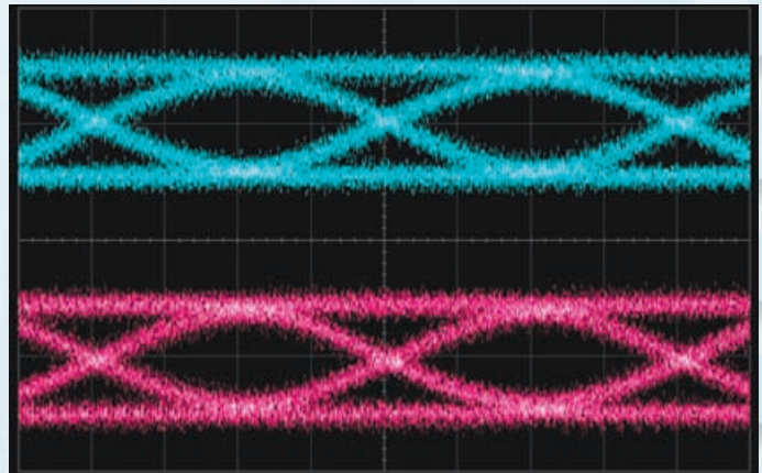
Signal transmission waveform TO-Package , 1.25Gbps NRZ , PRBS 2 7 -1
