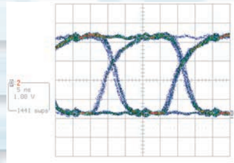
50Mbps受光波形 50Mbps receiver-output waveform
